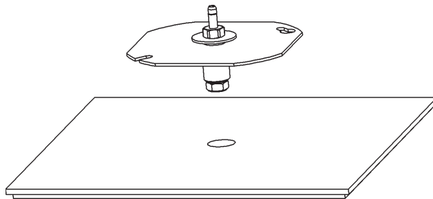
Fig. 11 Exploded view drawing of ceiling static pressure pickup port, BAPI ZPS-ACC05, showing how to mount in ceiling tile.
