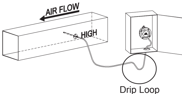
Fig. 2 Measuring static pressure in a duct with BAPI ZPS Pressure Transmitter mounted in a panel and BAPI ZPS-ACC07 in duct.
