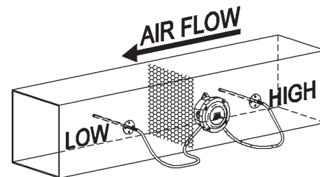
Fig. 3 Measuring air filter pressure drop with BAPI ZPS Pressure Transmitter mounted on a duct and two BAPI ZPS-ACC07 in duct.
