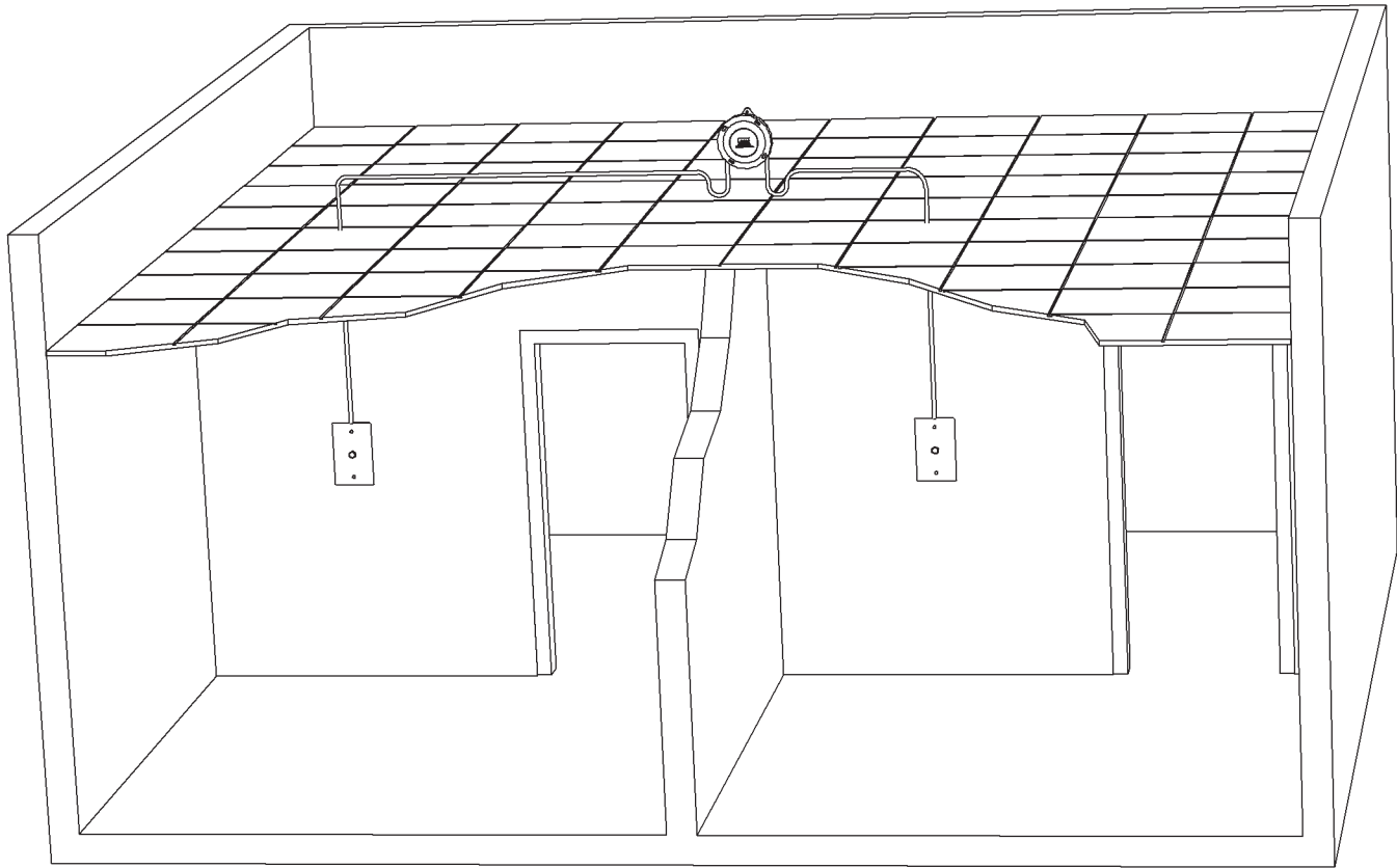
Fig. 10 Measuring static pressure differences between two rooms using two BAPI ZPS-ACC01 stainless steel wall plates and a BAPI ZPS Pressure Transmitter.
