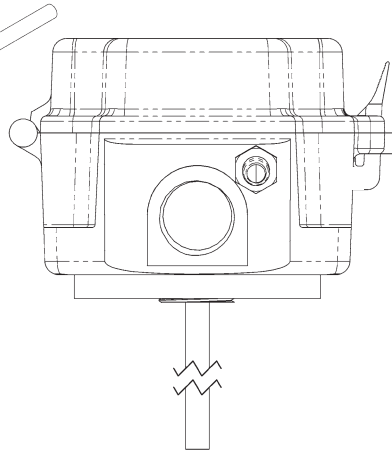
Fig. 2: End view of ZPS in a BAPI-Box with Attached Static Tube
