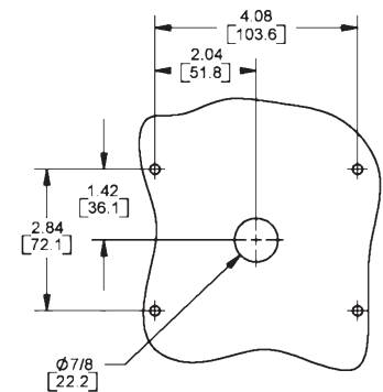
Fig. 1: Screw Hole Template. Drill center 7/8" hole for rear conduit entry on Rough Service Unit. Drill 1" hole for Aspiration Tube on Duct Unit
